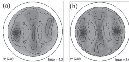
Fig. 3. Pole figure ( Al_{220} ) of the precursor material. (a) As-received samples; (b) After 1h at 565\text{ }^{\circ}\text{C} .
