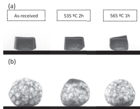
Fig. 4. Radioscopy images (cross section view) at two stages of the foaming process. (a) Semisolid expansion; (b) Final -liquid- expansion. Initial precursor shape is also indicated ( 5 \times 10\text{ mm}^2 ).
