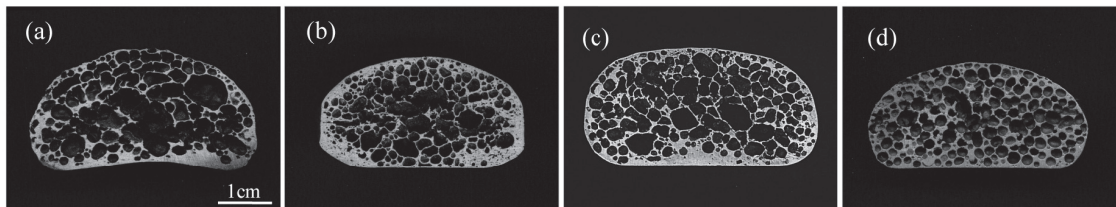
Fig. 5. Cross section of the foams produced after different heat treatments. Same foaming conditions: 710\text{ }^{\circ}\text{C} , 9min. (a) As-received material; (b) 500\text{ }^{\circ}\text{C} , 8h; (c) 535\text{ }^{\circ}\text{C} , 2h; (d) 565\text{ }^{\circ}\text{C} , 1h.
